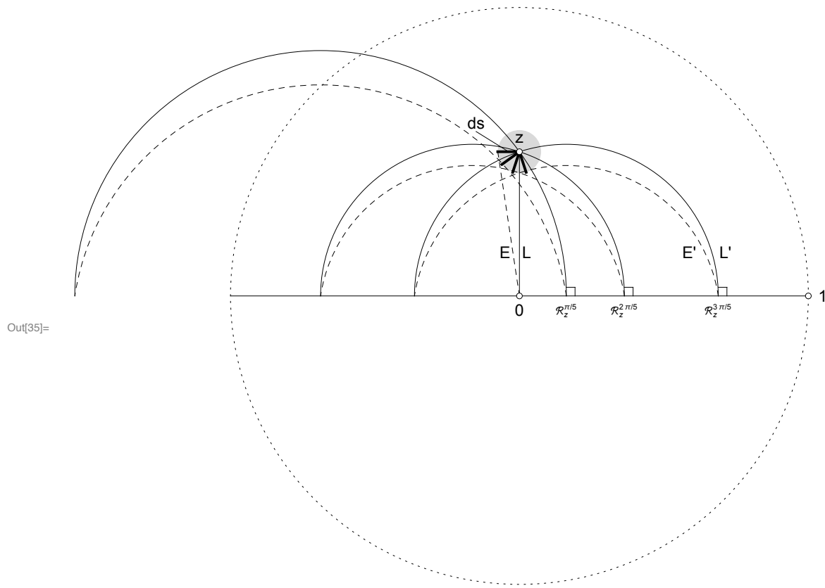
Figure 1. Poincaré Disc: Three rotations of \pi/5 Cf. Figure [36a], p. 318, Needham
